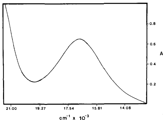
Figure 21. Expanded view of the {}^3(\delta \rightarrow \delta^*) transition of a single crystal of W_2(np)_2(O_2CET)_4 at 5 K.
