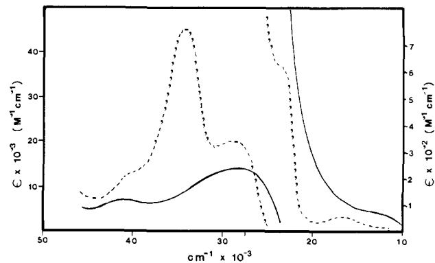
Figure 18. Comparison of the electronic absorption spectra of W_2(np)_2(O_2Cet)_4 (dashed line) and W_2(O_2Cet)_4 (solid line) in the region 10 000–50 000 cm^{-1} recorded in hexane at room temperature.
