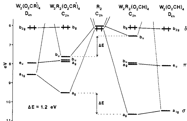
Figure 17. Qualitative interaction diagram comparing the experimental (left two columns) and calculated (right two columns) electronic structure of W_2(O_2CR')_4 and W_2R_2(O_2CR')_4 complexes. This diagram illustrates qualitatively the difference between experimental and calculated energies of \sigma type orbitals, represented by \Delta E .
