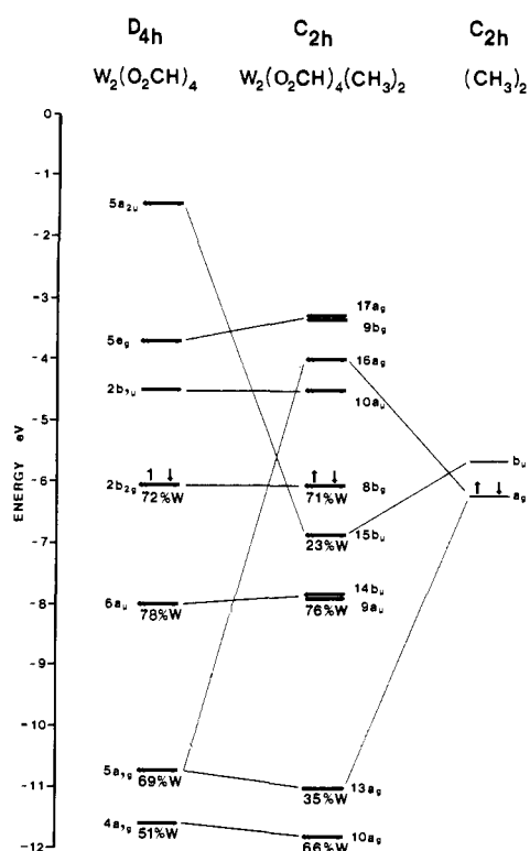
Figure 10. Results of the relativistic SCF-X \alpha -SW calculations on W_2(O_2CH)_4(CH_3)_2 . This diagram shows the correlation of the orbitals of W_2(O_2CH)_4(CH_3)_2 to those of W_2(O_2CH)_4 and (CH_3)_2 . Only those levels involved in W-W bonding or antibonding are shown. The HOMOs are denoted by use of spin-paired arrows (taken from ref 44).
