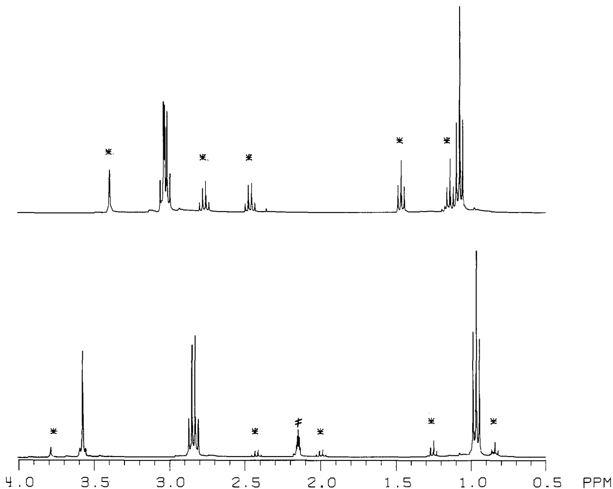
Figure 2. ^1\text{H} NMR spectra of \text{W}_2\text{Bz}_2(\text{O}_2\text{Ct})_4 in toluene- d_8 (bottom spectrum) and \text{CD}_2\text{Cl}_2 (top spectrum) showing the presence of two isomers, I and II, defined in the text, and the solvent dependence on the equilibrium concentrations of each. The proton signals denoted by an asterisk correspond to isomer II, and the residual protons in toluene- d_8 in the lower spectrum are denoted by a dagger. The spectra were recorded at 360 MHz and 22 ^\circ\text{C} . The \text{CH}_2\text{Ph} protons of isomer I in \text{CD}_2\text{Cl}_2 are partially obscured by the \text{O}_2\text{CCH}_2\text{CH}_3 signals.
