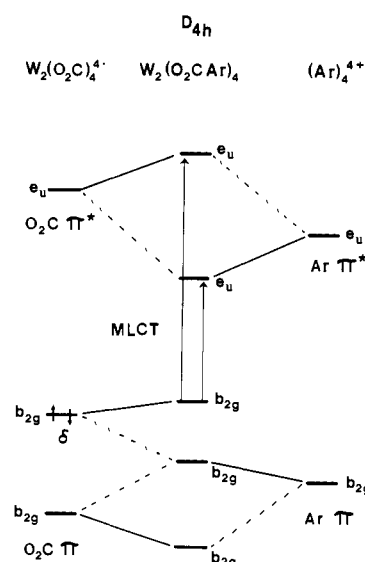
Figure 24. Schematic correlation diagram depicting the interaction between the arene \pi and \pi^* orbitals and the CO_2 \pi and \pi^* and M-M \delta orbitals in W_2(O_2CAr)_4 compounds in D_{4h} symmetry. Only the relevant b_{2g} and e_u orbitals are shown.
