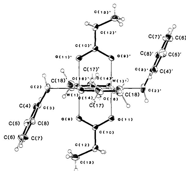
Figure 4. ORTEP drawing of the \text{W}_2\text{Bz}_2(\text{O}_2\text{Ct})_4 molecule showing the atom number scheme used in the tables.
