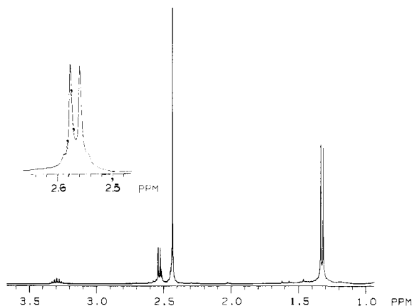
Figure 1. ^1\text{H} NMR spectrum of \text{W}_2(i\text{-Bu})_2(\text{O}_2\text{CMe})_4 in benzene- d_6 at 360 MHz, 22 °C. Inset shows the methylene protons of the W- i -Bu moiety with coupling to both the neighboring methine proton and ^{183}\text{W} nuclei, I = 1/2 , 14.5% natural abundance.
