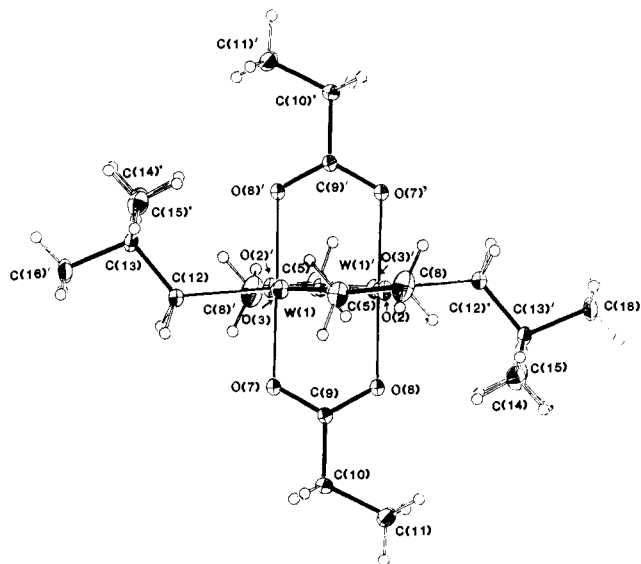
Figure 5. ORTEP drawing of the W_2(np)_2(O_2CET)_4 molecule showing the atom number scheme used in the tables.
