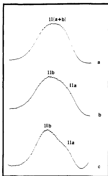
Figure 13. Expanded views of the ionization labeled II in Figure 12 showing two distinct components for W_2(np)_2(O_2CR')_4 where R' = \text{Me} (a), H (b), and \text{CF}_3 (c).
