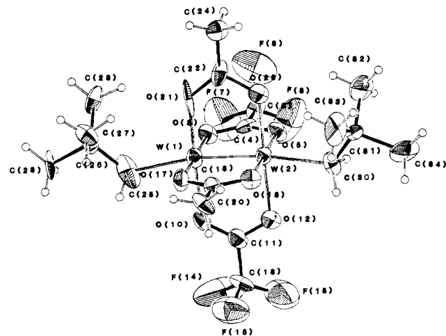
Figure 8. ORTEP view of the W_2(np)_2(O_2CMe)_2(O_2CCF_3)_2 molecule showing the atom number scheme used in the tables.
