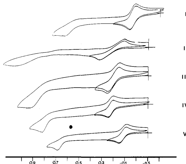
Figure 11. Cyclic voltammograms recorded in CH_2Cl_2 referenced against a Ag/Ag^+ electrode at 200 mV/s for W_2(O_2CEt)_4 (I), W_2(np)_2(O_2CMe)_4 (II), W_2(np)_2(O_2CEt)_4 (III), W_2(np)_2(O_2CPh)_4 (IV), and W_2(np)_2(O_2CC_6H_4-p-OMe)_4 (V).
